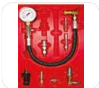
Compression Tester 1000 Psi & 70 Bar | 420mm Hose
