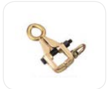
Box Clamp - Two Way 6 Ton Straight | 2 Ton Cross
